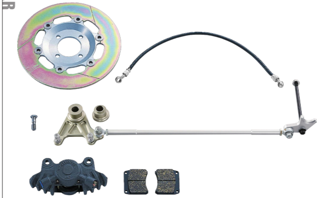
JB-POWER Rear Floating Brake Kit ¥ 184,600.- [Cast Iron Disc φ250, CP2696 Caliper, Brake Pads, Caliper Bracket [Collar included], Torque Rod, Torque Rod Anker, Stainless Mesh Brake Hose, Stainless Fitting, Banjo Bolt]
