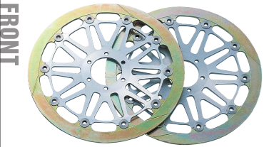
JB-POWER Cast Iron Front Brake Disc φ320 6 · 2/4 POT 1PCS ¥ 75,000.-
